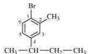
1-Bromo-4-sec-butyl-2-methylbenzene
