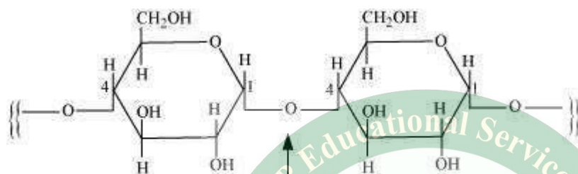
\alpha -Link Amylose
