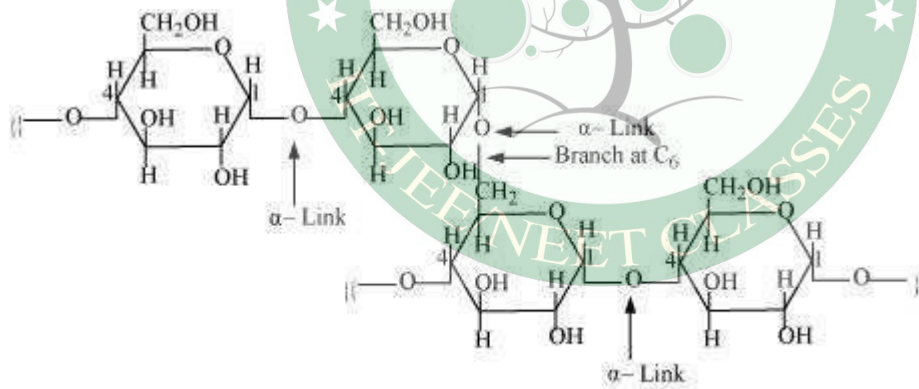
Amylopectin
